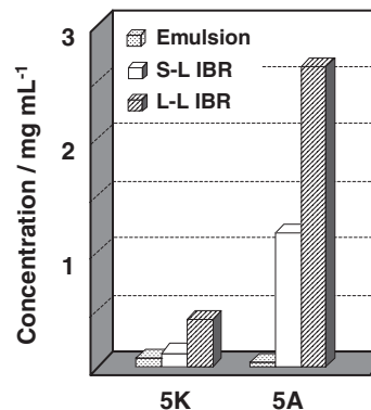
Figure 4. Comparison of 5-decanol and 5-decanone production with R. oryzae R-38-8 among emulsion, S-L IBR, and L-L IBR systems. 5K , 5-decanone; 5A , 5-decanol. While the emulsion system was conducted at 25 °C with agitation (300 rpm) for 5 days, the S-L and L-L IBR systems were statically conducted at 25 °C.
