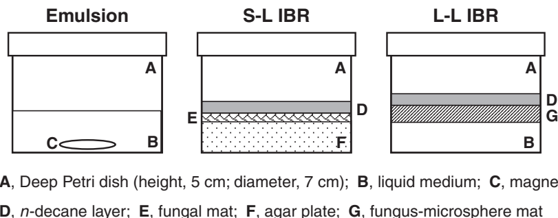
Figure 2. Schematic diagrams of emulsion, S–L IBR, and L–L IBR systems. All systems are shown as vertical sections.
